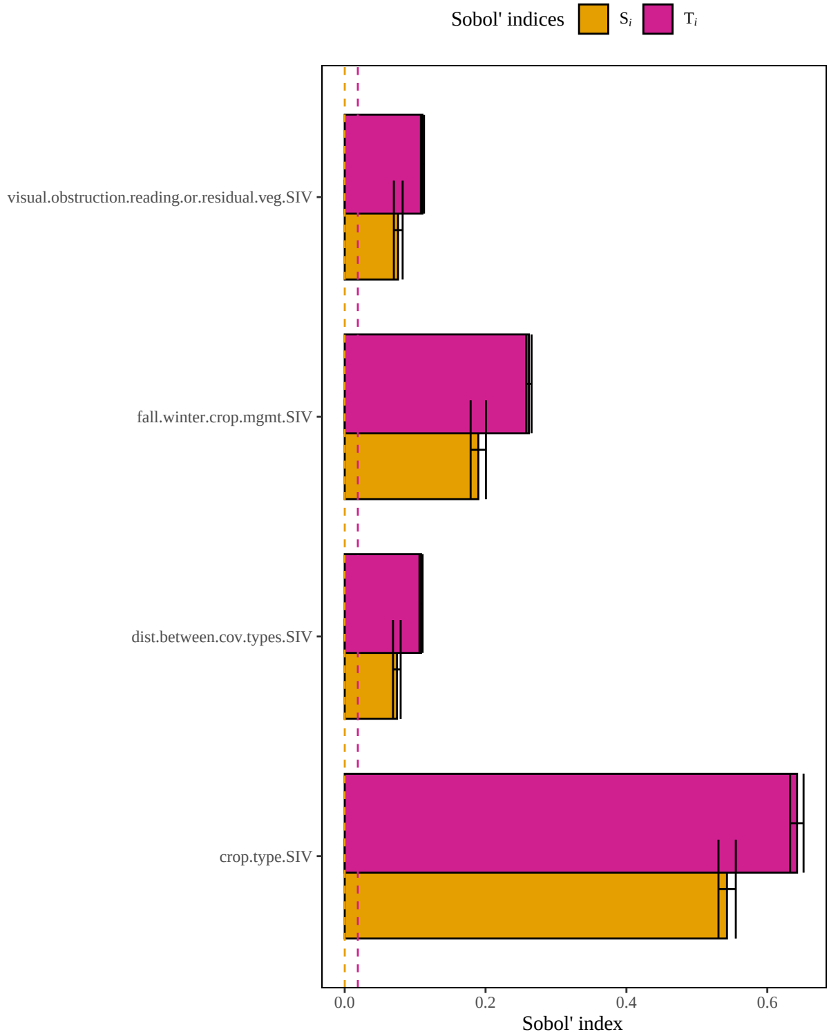
Figure 5. Results of a sensitivity analysis for the greaterprairiechickenHarvested model based on a geometric mean structure. Dashed lines represent baseline numerical approximation error for S_i and T_i ( i.e. , dummy variables).
