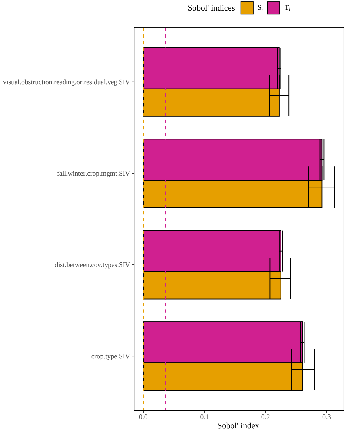
Figure 4. Results of a sensitivity analysis for the greaterprairiechickenHarvested model based on an arithmetic mean structure. Dashed lines represent baseline numerical approximation error for S_i and T_i ( i.e. , dummy variables).
